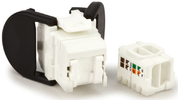
V250U CAT.6 UTP Three-Way Entry Jack XF500006424
